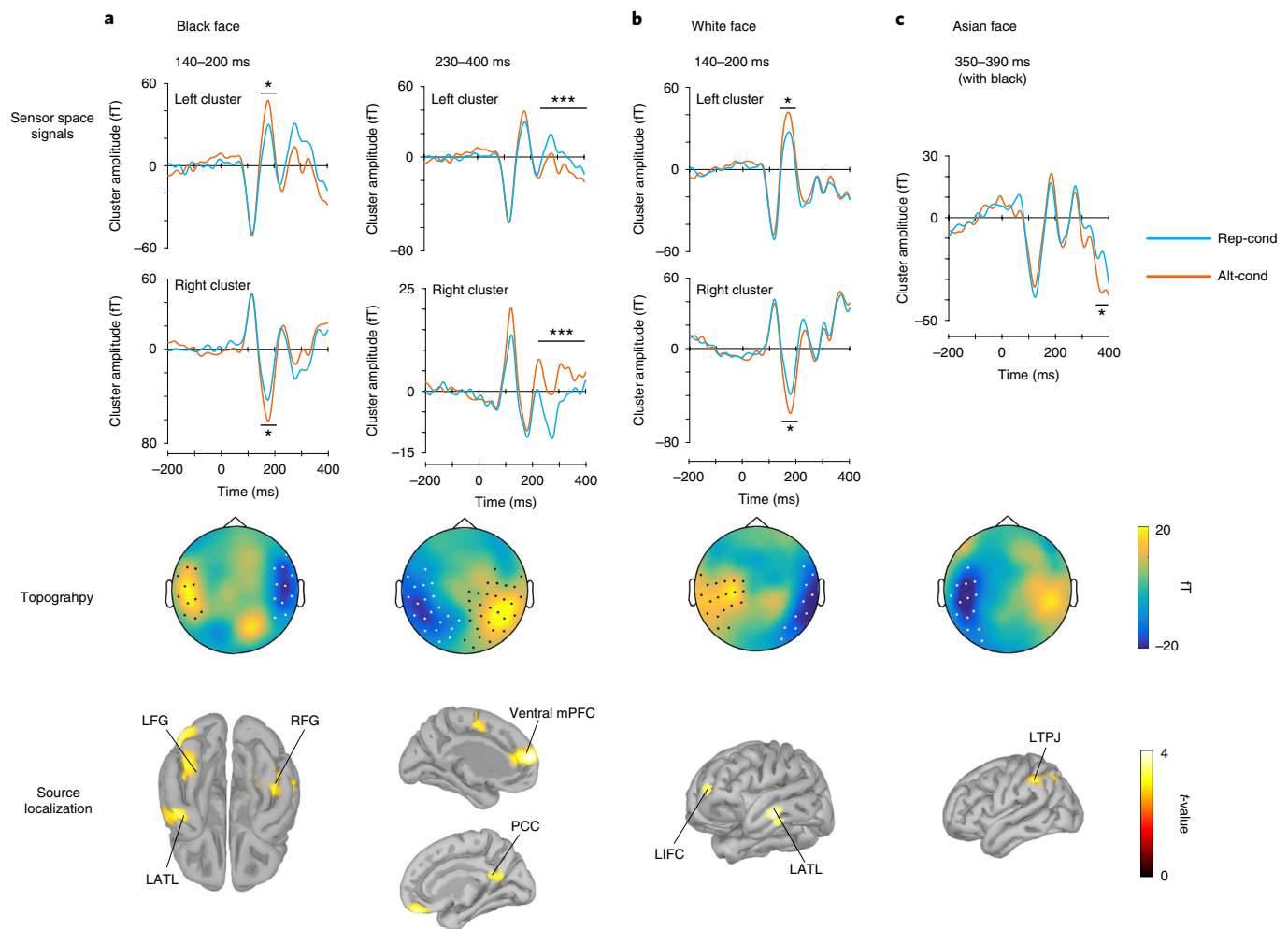
Fig. 6 | MEG results of Chinese participants in experiment 6. a–c, Results relate to black (a), white (b) and Asian faces (c). The upper panels illustrate the grand average sensor-space MEG signals averaged across the sensors in significant clusters ( N=26 ). The middle panels show topographies of the RS effects (Alt-Cond minus Rep-Cond) in each time window (dots represent sensors contributing to the significant clusters). The lower panels show source brain regions that contribute to the RS effects on sensor-space signals in each time window. The RS of MEG signals to all faces were identified using a threshold cluster of P < 0.025 (two-tailed for sensor-space and one-tailed for source-space) and corrected for multiple comparisons. A lenient threshold of 30 contiguous vertices, P values < 0.005 uncorrected, were used only for source-space visualization.
