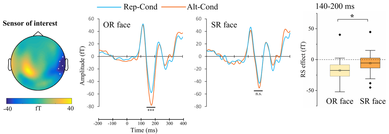
Extended Data Fig. 8 | Results of MEG sensor-space signals in experiment 6. The left panel shows the magnetometer sensors that showed the strongest neural responses at 140–200 ms across all conditions ( p < 0.05 , FDR corrected). The middle panel shows mean MEG responses over these sensors to OR-faces and SR-faces. The right bar charts illustrate the mean RS effects in sensor-space MEG signals (Alt-Cond > Rep-Cond) by showing quartiles (boxes), means (square inside boxes), medians (horizontal lines inside boxes), maximum and minimum excluding outliers (whiskers), and outliers (diamonds). ANOVAs of the mean sensor-space magnetic responses at 140–200 ms confirmed a larger RS effect for OR-(collapsing Black and White faces) than SR-(Asian) faces ( N=26 ; F(1,25) = 6.663 , p = 0.016 , \eta_p = 0.210 , 90% CI = 0.02, 0.41).
