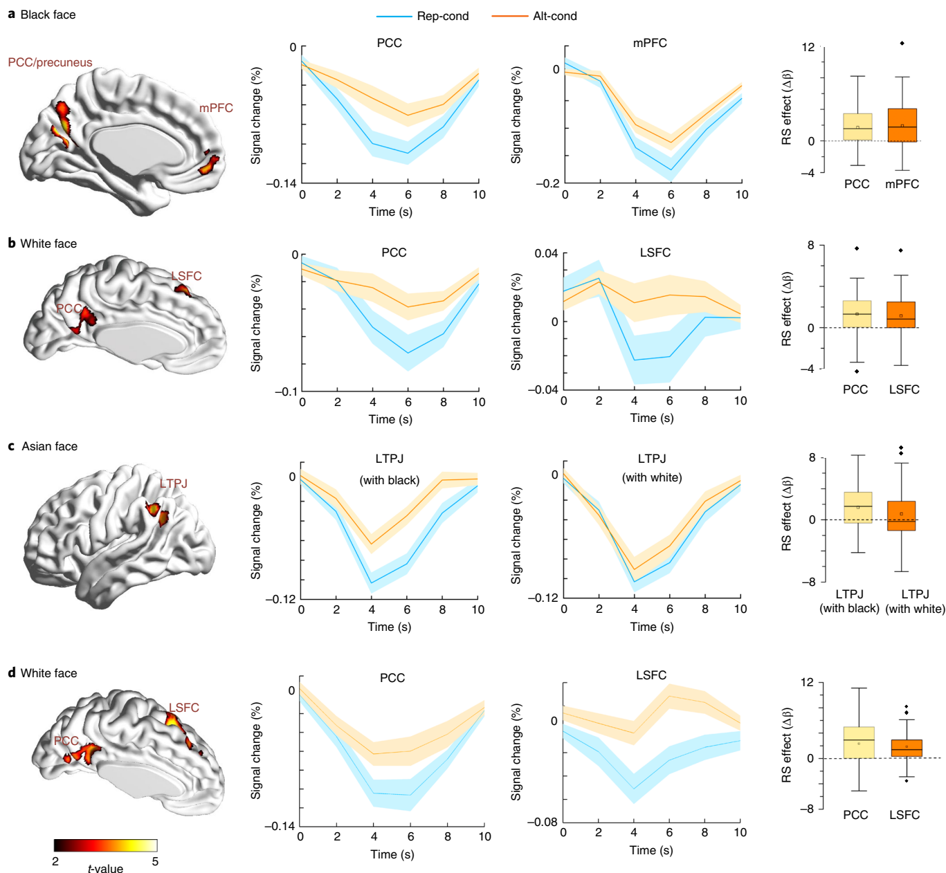
Fig. 5 | fMRI results of Chinese participants in experiments 5a and 5b. a–c , Results of experiment 5a ( N=55 ; 2 participants were excluded from analyses due to excessive head movement). d , Results of experiment 5b ( N=40 ). For all panels, the left column shows brain regions in which significant RS of BOLD responses occurred. The middle column illustrates time courses ( \pm s.e.m. shown as shading around the mean trace) of BOLD responses in these brain regions in the Alt-Cond and the Rep-Cond. The box plots in the right column illustrate the mean RS effects indexed by differences in \beta -values (Alt-Cond minus Rep-Cond) in each brain region. The plots show the quartiles (boxes), means (square inside boxes), medians (horizontal lines inside boxes), maximum and minimum excluding outliers (whiskers), and outliers (diamonds). RS effects on BOLD responses in a , c and d were identified and visualized using a combined voxel level threshold of P < 0.001 uncorrected and a cluster level of P < 0.05 FWE-corrected. RS effects on BOLD responses in b were explored and visualized using a threshold of P < 0.005 uncorrected and a voxel number > 70 .
