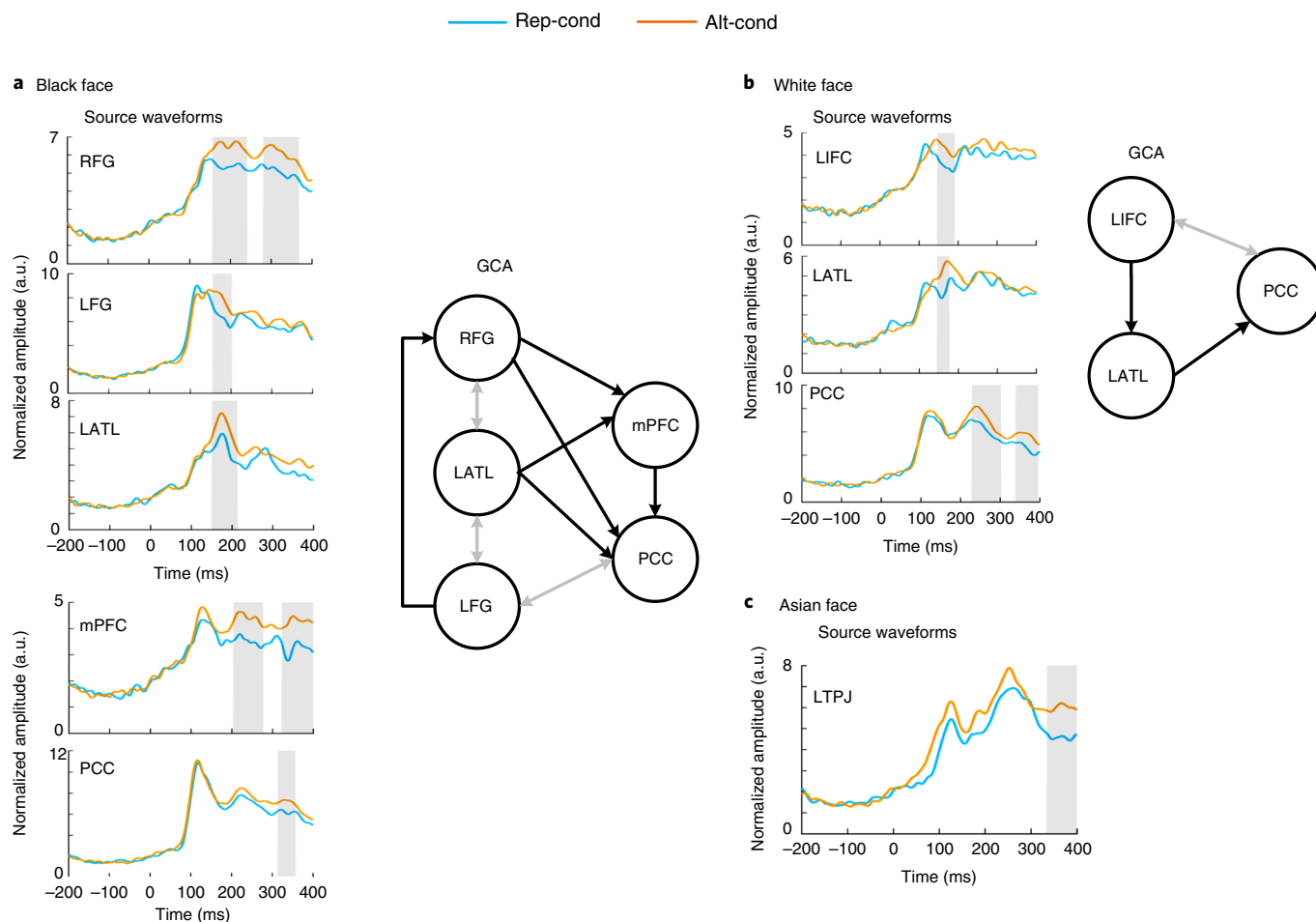
Fig. 7 | Dynamic neural models of racial categorization revealed in experiment 6. a–c , RS effects on source-space MEG signals and dynamic models of categorization processes for black ( a ), white ( b ) and Asian faces ( c ). The grand average of source-space MEG signals in the brain regions included in the GCA are shown on the left of each panel, and dynamic models of categorization processes are shown on the right of each panel (note, there is no model for Asian faces). Time windows showing reliable RS effects on source-space MEG signals are marked with grey bars ( N=26 , cluster P values < 0.05 , FDR-corrected). Black lines and arrows in the dynamic models indicate unidirectional causal influences. Grey lines and arrows indicate bidirectional causal influences. Significance was assessed using a threshold of P < 0.05 , Bonferroni-corrected for GCA. a.u., arbitrary unit.
