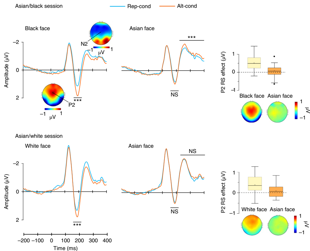
Fig. 3 | Results of Chinese participants in experiment 2. Left: ERPs to OR (black and white) and SR (Asian) faces at frontal/central electrodes (the x axis at the bottom of the figure is applicable to all the ERP charts). Right: box plots illustrating the RS effects on P2 amplitudes (that is, the difference in P2 amplitudes between the Alt-Cond and the Rep-Cond) to OR faces and SR faces. The plots show the quartiles (boxes), means (square inside boxes), medians (horizontal lines inside boxes), maximum and minimum excluding outliers (whiskers), and outliers (data points higher or lower than 1.5-times the quartile (25th and 75th percentile) values) (diamonds). The voltage topographies show locations of the maximum P2 and N2 amplitudes and the maximum RS effect on P2 amplitudes over the frontal/central regions for both black and white faces. There was significant RS of the P2 amplitudes to black faces ( N=36 , F(1,35)=56.91 , P<0.001 , \eta_p^2=0.619 , 90% CI=0.43, 0.72) and white faces ( N=31 , F(1,30)=23.47 , P<0.001 , \eta_p^2=0.439 , 90% CI=0.21, 0.59), but not to Asian faces (Asian/black sessions: F(1,35)=2.75 , P=0.106 , \eta_p^2=0.073 , 90% CI=0, 0.23; Asian/white sessions: F(1,30)=2.29 , P=0.141 , \eta_p^2=0.071 , 90% CI=0, 0.24). There was significant RS of the N2 amplitude to Asian faces in Asian/black sessions ( F(1,35)=12.32 , P=0.001 , \eta_p^2=0.260 , 90% CI=0.07, 0.43) but not in Asian/white sessions ( F(1,30)=1.94 , P=0.174 , \eta_p^2=0.061 , 90% CI=0, 0.23). *** P\leq 0.001 .
