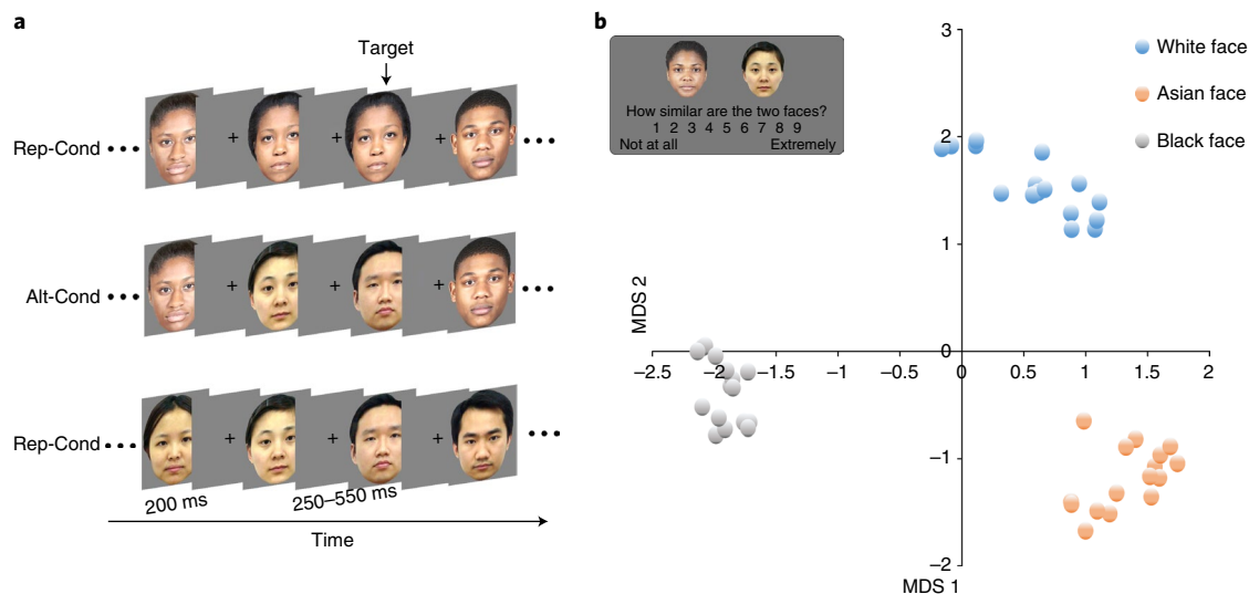
Fig. 1 | Stimuli and behavioural results. a , Illustration of the stimuli and procedures in the Rep-Cond and the Alt-Cond in experiment 1a. There were equal numbers of target faces in the Alt-Cond and the Rep-Cond. b , Stimuli, procedures and results of Chinese participants in the pilot experiment. Asian, black and white faces were clustered in a two-dimensional face-space built on the basis of similarity rating scores in the pilot experiment ( N=55 ). Black faces ( M=0.51 ) were more densely clustered than white ( M=1.38 ) and Asian ( M=1.25 ) faces. F(2,45)=45.59 , P<0.001 , \eta_p^2=0.670 , 90% CI=0.51, 0.74; post hoc analyses. Bonferroni-corrected: black versus Asian: P<0.001 , CI=-0.99, -0.50; black versus white: P<0.001 , CI=-1.12, -0.63; Asian versus white: P=0.601 , CI=-0.12, 0.37. The distance between Asian and black clusters ( M=3.51 ) was longer than that between Asian and white clusters ( M=3.18 ) ( t(30)=6.63 , P<0.001 , Cohen's d=2.34 , CI=0.23, 0.43) in the face space. MDS, multidimensional space. Face images reproduced from refs. 13 and 75 .
