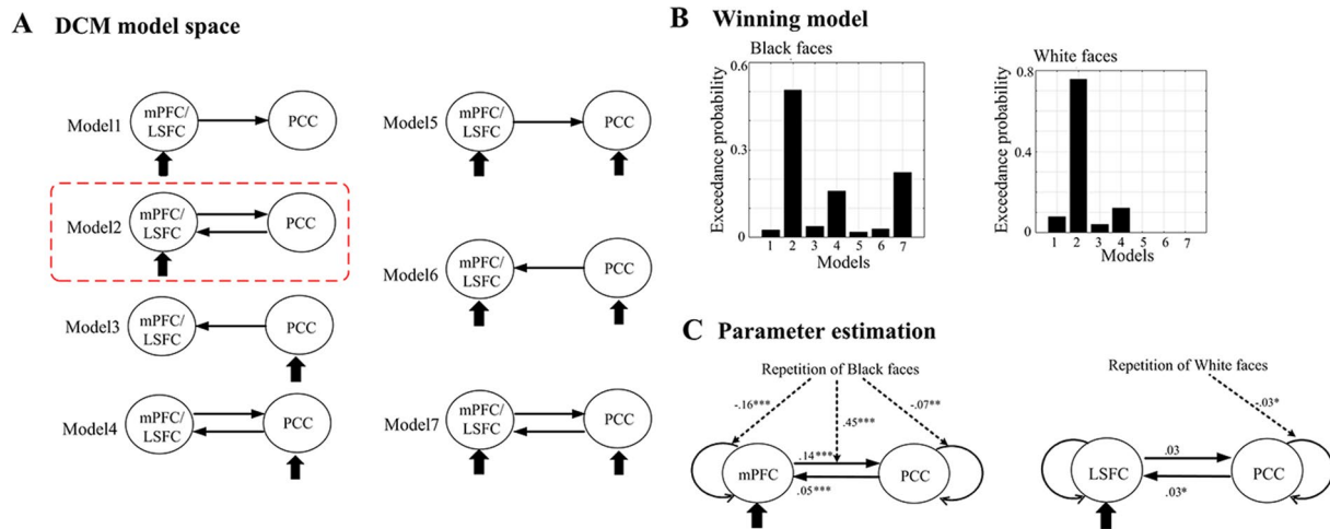
Extended Data Fig. 6 | Model structures and results of the DCM analysis in experiment 5a. (a) Illustration of individual models in the DCM model space. The models were different in the region that driving vision input were assigned to and the intrinsic connectivity between regions. Only the intrinsic connectivity between brain regions and the driving visual input were plotted. The modulation effect of on each intrinsic connectivity and the intrinsic connectivity within each regions of the single models were omitted. (b) The exceedance probabilities of single models of Black and White faces. Model 2 marked inside the red square had the highest exceedance probability for both Black and White faces. (c) Strength of the intrinsic and modulatory connectivity estimated based on Model 2 for Black and White faces, respectively. Repetition of Black faces significantly modulated within-region connectivity in both mPFC and PCC ( N=53 ; mPFC to mPFC: t(52) = -3.06 , p = 0.003 , Cohen's D = 0.42 , 95% CI = -0.27, -0.06 , PCC to PCC : t(52) = -3.34 , p = 0.002 , Cohen's D = 0.46 , 95% CI = -0.12, -0.03 ) and between-region connectivity from mPFC to PCC ( t(52) = 6.12 , p < 0.001 , Cohen's D = 0.84 , 95% CI = 0.30, 0.60 ). By contrast, repetition of White faces only significantly modulated within- region connectivity for PCC ( t(52) = -2.10 , p = 0.041 , Cohen's D = 0.29 , 95% CI = -0.06, -0.001 ). * p < 0.05 , ** p < 0.01 , *** p < 0.001 .
