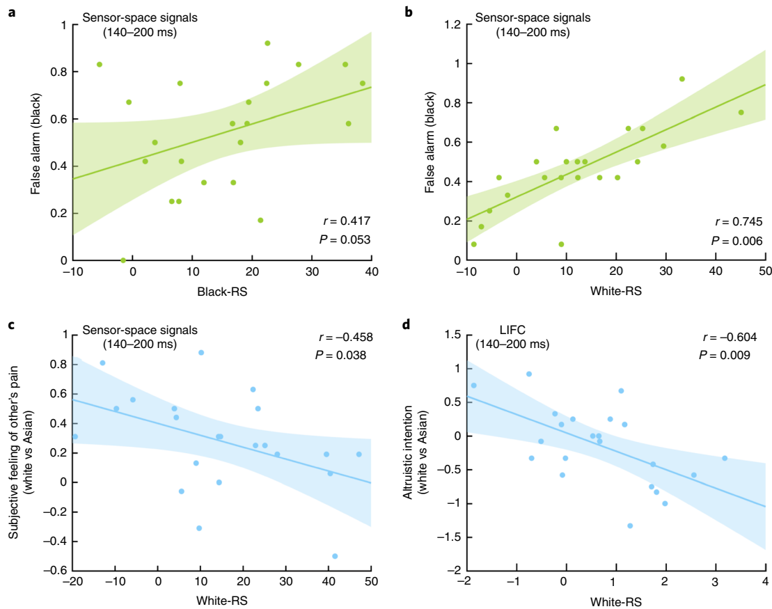
Fig. 8 | Coupling between neural categorization of OR faces and racial biases in cognition and altruistic intention in experiment 6. a, b , Correlations between early RS effects on sensor-space MEG signals to black ( a ) and white ( b ) faces and false alarm rates in the face recognition task. Greater RS of sensor-space MEG signals to white faces at 140–200 ms predicted more false alarms when recognizing old/new white faces ( N = 22 , r = 0.745 , P = 0.006 , 95% CI = 0.42, 0.92, FDR-corrected). A similar trend was observed for black faces ( r = 0.417 , P = 0.053 , 95% CI = -0.05, 0.78, FDR-corrected). c , The correlation between early RS effects on sensor-space MEG signals to white faces and subjective feelings of pain of white (versus Asian) faces. Stronger RS of sensor-space MEG signals to white faces at 140–200 ms predicted weaker subjective feelings of pain of white (versus Asian) faces ( N = 22 , r = -0.458 , P = 0.038 , 95% CI = -0.77, -0.04, FDR-corrected). d , The correlation between RS of source-space LIFC responses to white faces and altruistic intentions to help white (versus Asian) individuals who suffer from painful stimulations. Stronger RS to white faces in LIFC predicted less intention to help white (versus Asian) models ( N = 22 , r = -0.604 , P = 0.009 , 95% CI = 0.22, 0.81, FDR-corrected).
