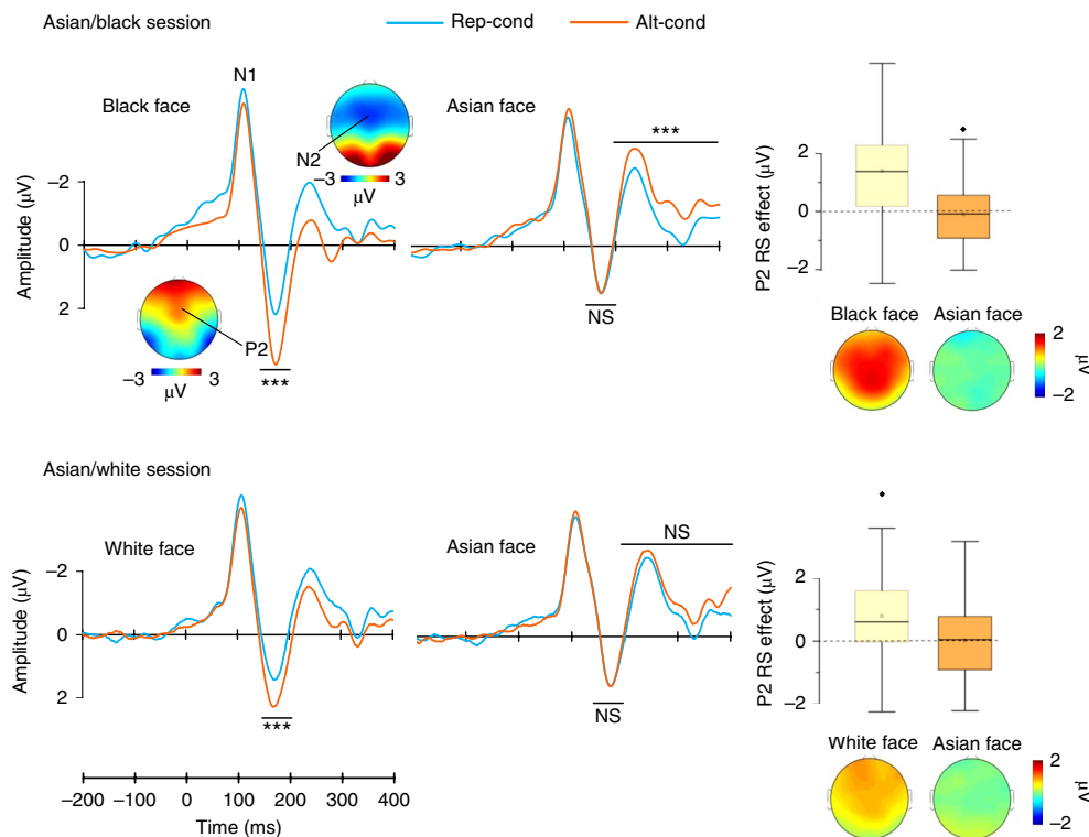
Fig. 2 | ERP results of Chinese participants in experiment 1a. Left: ERPs to OR faces and SR faces at frontal/central electrodes (the x axis at the bottom of the figure is applicable to all the ERP charts). Right: box plots illustrating the RS effects (that is, decreased amplitudes in the Rep-Cond compared with the Alt-Cond) on P2 amplitudes to OR and SR faces. The plots show the quartiles (boxes), means (square inside boxes), medians (horizontal lines inside boxes), maximum and minimum excluding outliers (whiskers), and outliers (data points higher or lower than 1.5-times the quartile (25th and 75th percentile) values) (diamonds). The voltage topographies show locations of the maximum P2 and N2 amplitudes and maximum RS effects on P2 amplitudes over the frontal/central regions for both black and white faces. There was significant RS of P2 amplitudes to black and white faces ( N=38 , F(1,37)=31.56 and 13.50 , P<0.001 and P=0.001 , \eta_p^2=0.460 and 0.267 , 90% CI=(0.25, 0.59) and (0.08, 0.43), respectively), but not to Asian faces (Asian/black and Asian/white sessions: F(1,37)=0.32 and 0.012 , P=0.576 and P=0.912 , \eta_p^2=0.009 and 0.000 , 90% CI=(0, 0.11) and (0, 0.03), respectively). There was significant RS of N2 amplitudes to Asian faces in Asian/black sessions ( F(1,37)=18.56 , P<0.001 , \eta_p^2=0.334 , 90% CI=0.13, 0.49) but not in Asian/white sessions ( F(1,37)=1.98 , P=0.167 , \eta_p^2=0.051 , 90% CI=0, 0.19). NS, not significant, ***P\leq 0.001 .
