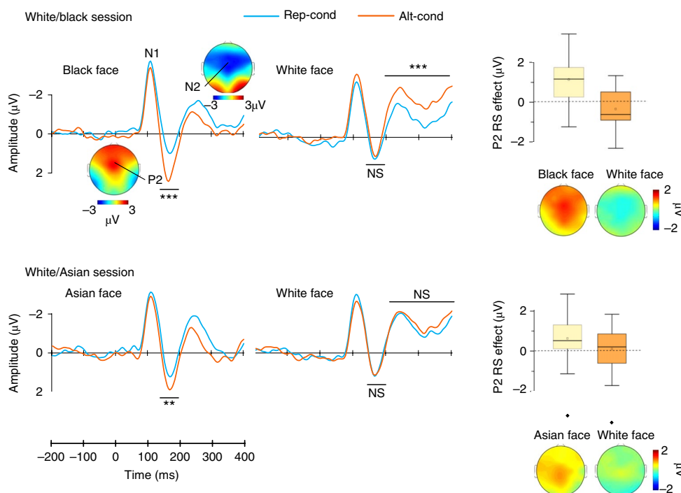
Fig. 4 | ERP results of white participants in experiment 3. Left: ERPs to OR faces and SR faces at frontal/central electrodes (the x axis at the bottom of the figure is applicable to all the ERP charts). Right: box plots illustrating the RS effects on P2 amplitudes to OR and SR faces. Plots show the quartiles (boxes), means (square inside boxes), medians (horizontal lines inside boxes), maximum and minimum excluding outliers (whiskers), and outliers (diamonds). The voltage topographies show locations of the maximum P2 and N2 amplitudes and the maximum RS effect on P2 amplitudes over the frontal/central regions for both black and Asian faces. There was significant RS of the P2 amplitudes to black faces ( N=32 , F(1,31)=32.23 , P<0.001 , \eta_p^2=0.510 , 90% CI=0.28, 0.64) and Asian faces ( N=35 , F(1,34)=9.81 , P=0.004 , \eta_p^2=0.224 , 90% CI=0.05, 0.40), but not to white faces (white/black sessions: ( F(1,31)=3.37 , P=0.076 , \eta_p^2=0.098 , 90% CI=0, 0.27; white/Asian sessions: F(1,34)=0.31 , P=0.582 , \eta_p^2=0.009 , 90% CI=0, 0.12). There was significant RS of the N2 amplitude to white faces in white/black sessions ( F(1,31)=19.40 , P<0.001 , \eta_p^2=0.385 , 90% CI=0.16, 0.54), but not in white/Asian sessions ( F(1,34)=2.69 , P=0.110 , \eta_p^2=0.073 , 90% CI=0, 0.23. ** P<0.01 ; *** P<0.001 ).
